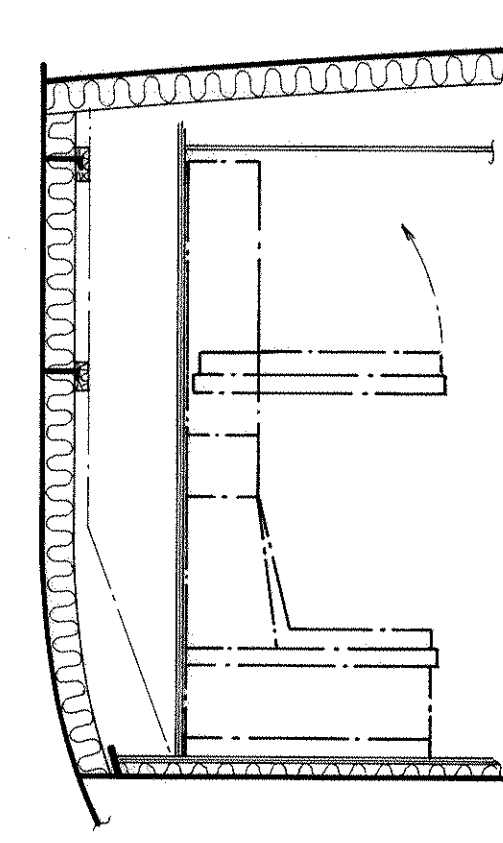
SNIT H-H
