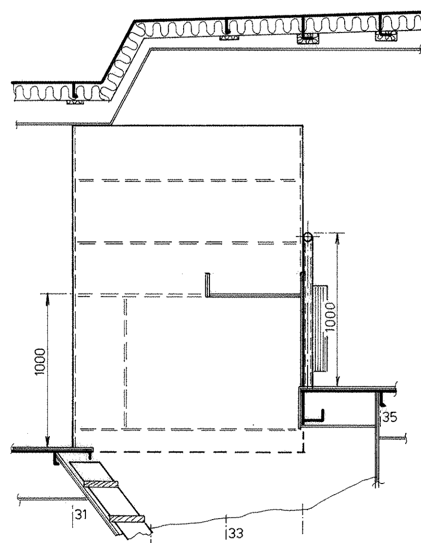
SNIT C - C
