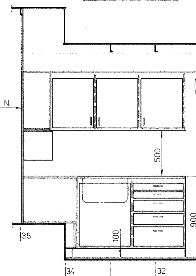
SNIT H-H
