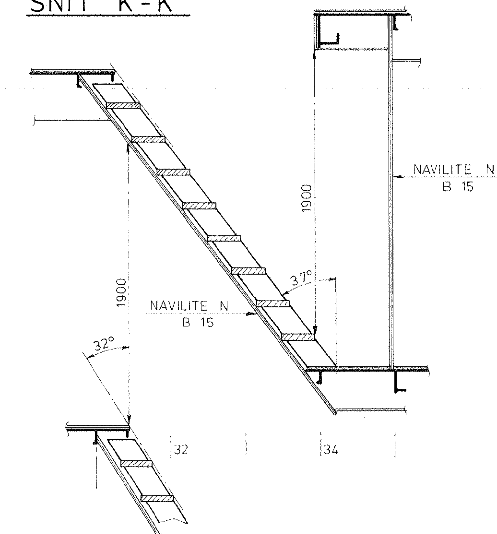
SNIT K-K
