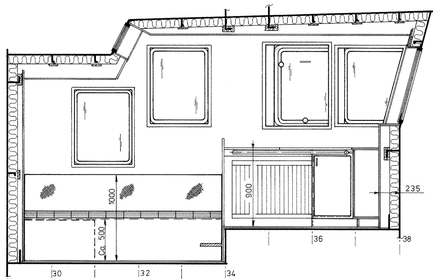
SNIT A - A
