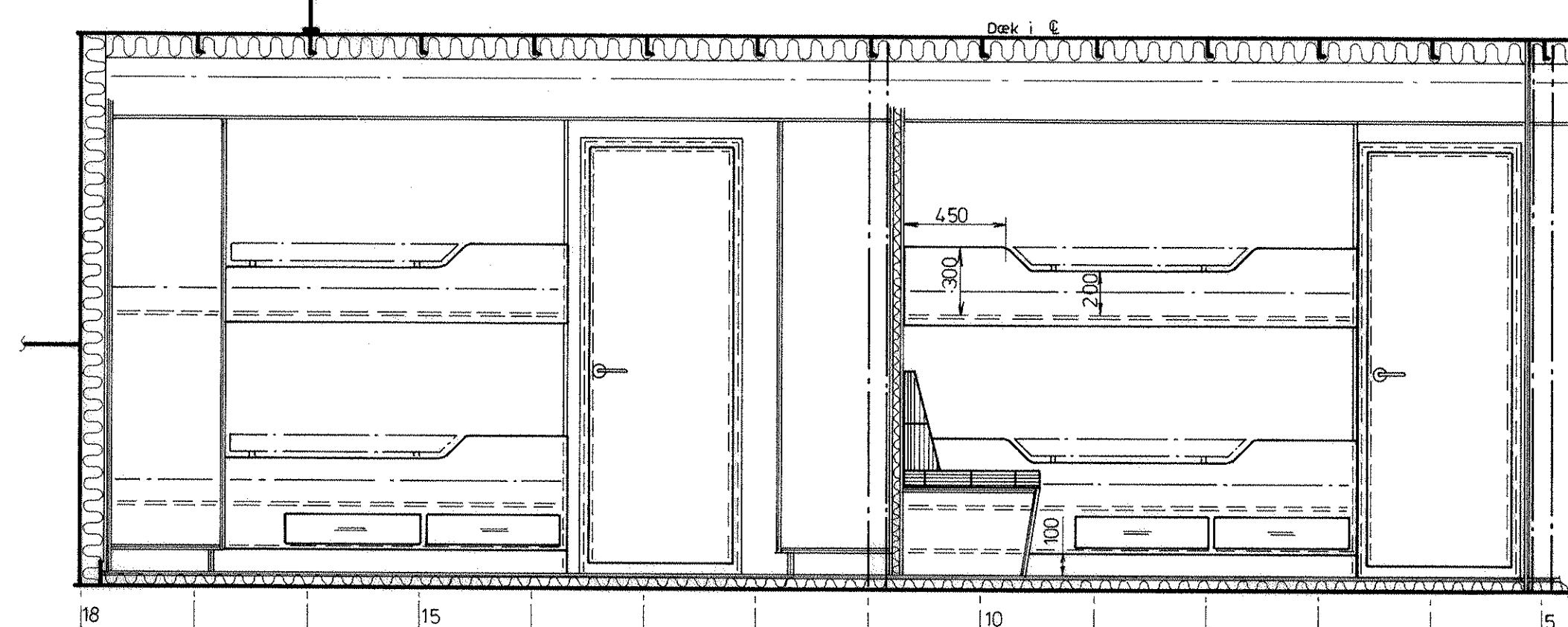
SNIT H-H
