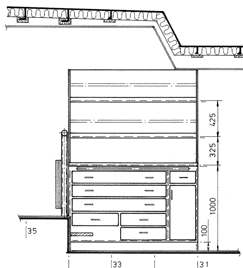
SNIT D - D
